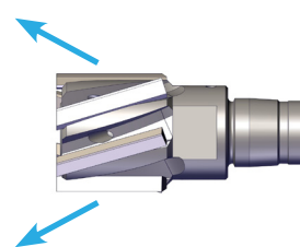
SERIES 5700: Left hand helical flutes Radial coolant
