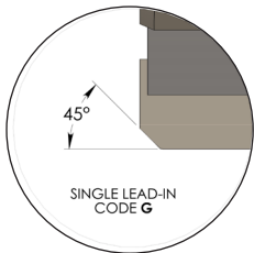
Lead-in 45° for standard speed
