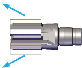
SERIES 5400: Straight flutes Radial coolant
